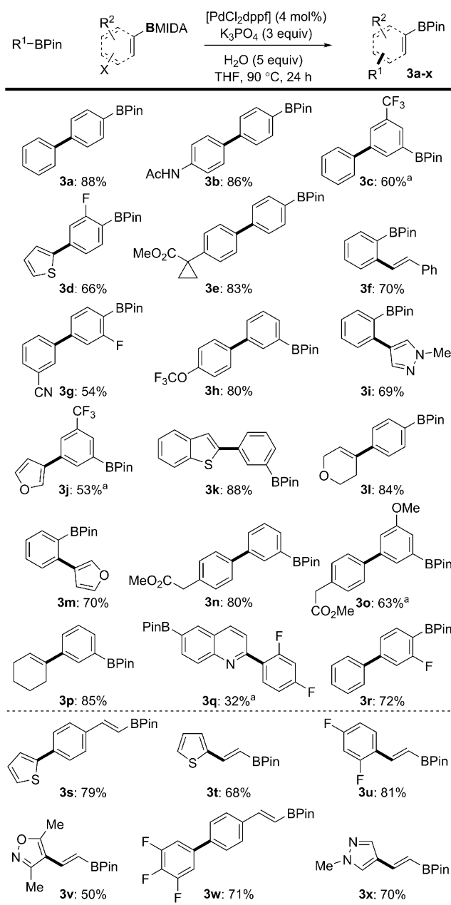
Figure 2. Scope of the formal homologation reaction with aryl boronic acid MIDA esters. All yields are those of the isolated products. X = Cl, Br, I. [a] Using \text{Pd}(\text{OAc})_2 (4 mol%) and SPhos (8 mol%). [11]
